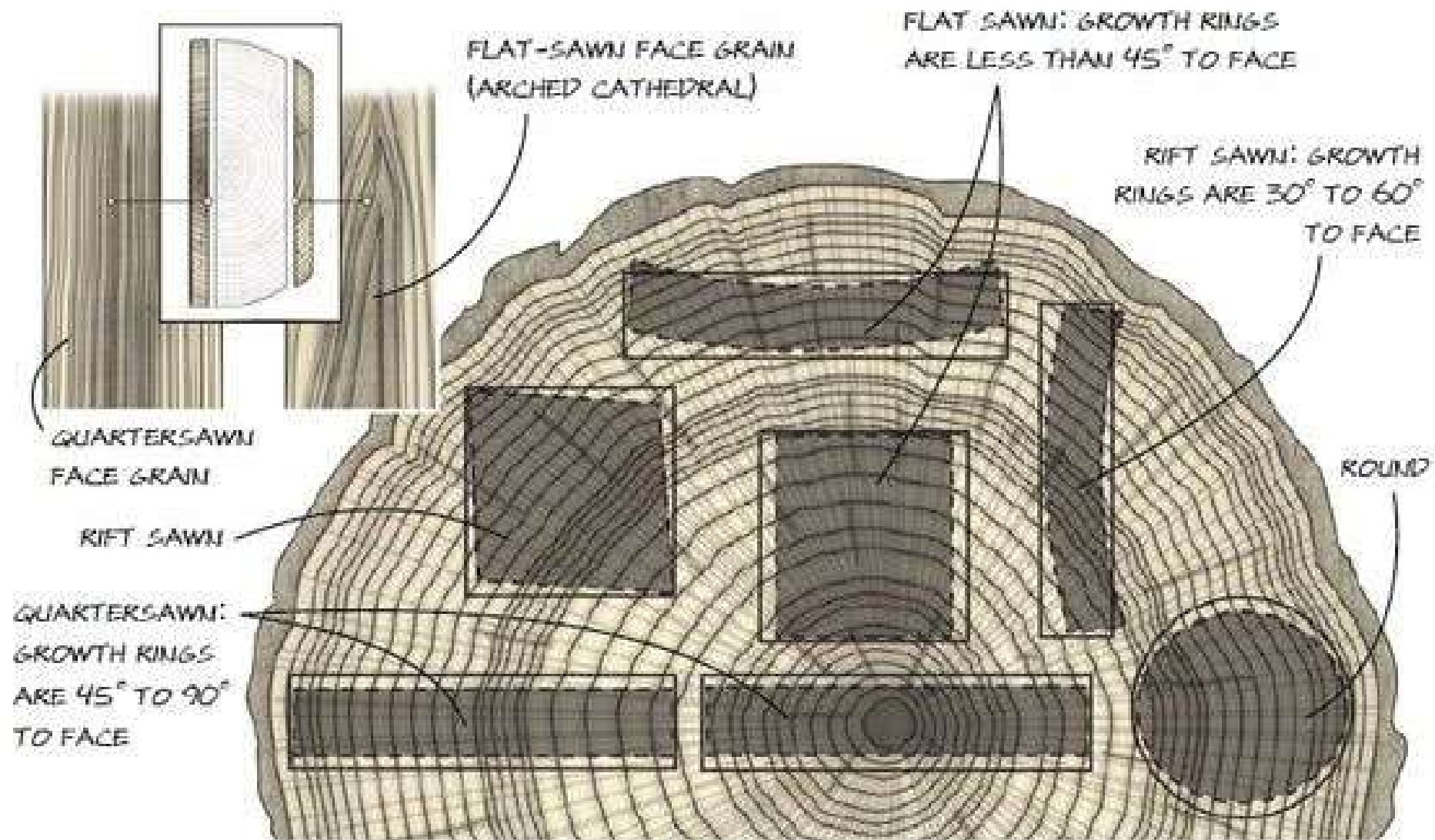
TYPE OF LUMBER CUT AND SHRINKAGE
